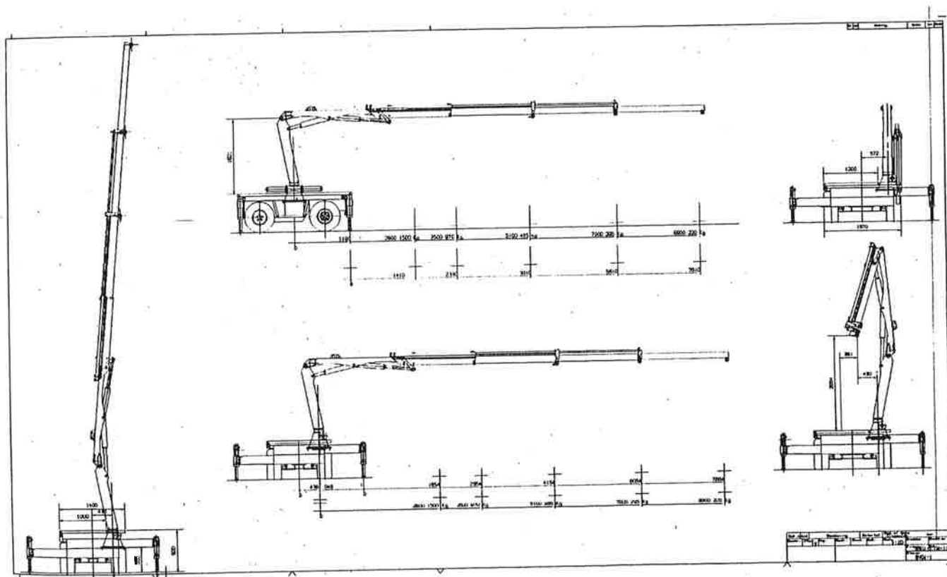
Figur 2.0.1 Ritning TEMOVAGNEN
